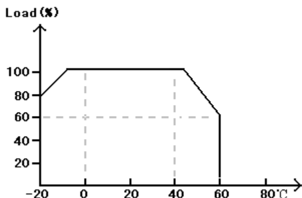
Temperature- load curve
